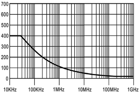
Fig. 1: Derating curve
